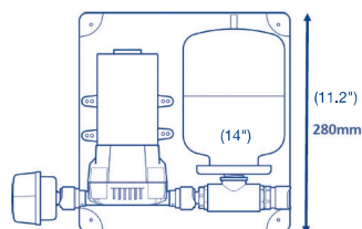
PLAN VIEW
